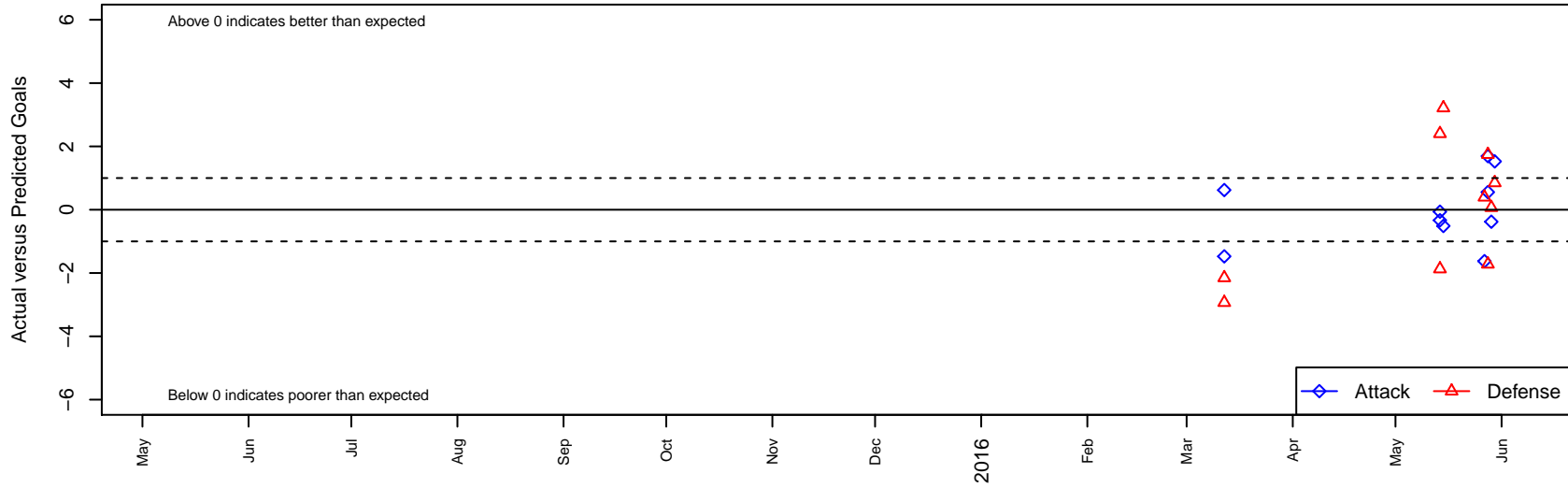
PVSC United Sounders B02 Dots are actual minus expected GF (blue circles) and GA (red triangles). Blue line is smoothed change in attack strength. Red is smoothed change in defense strength.
